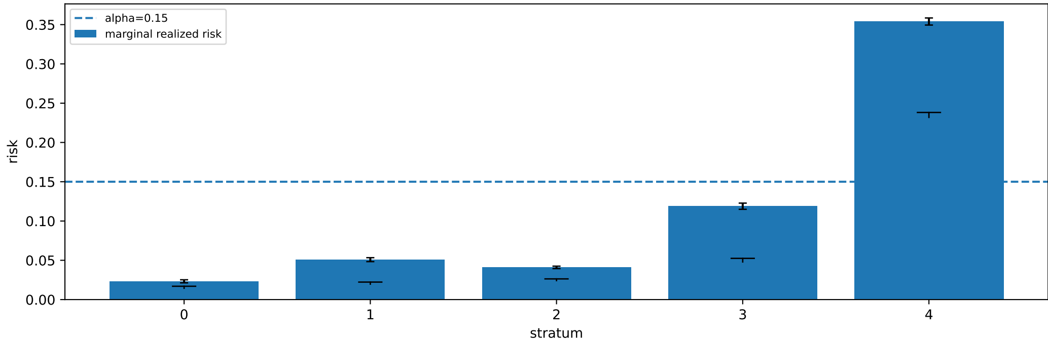
F2 per-stratum marginal risk -- tabular-MiniBooNE[margin] ts0 greedy lambda_ref=0.9
